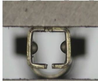
Current terminal from Shanghai. Meets Molex specifications for fit, form and function.
